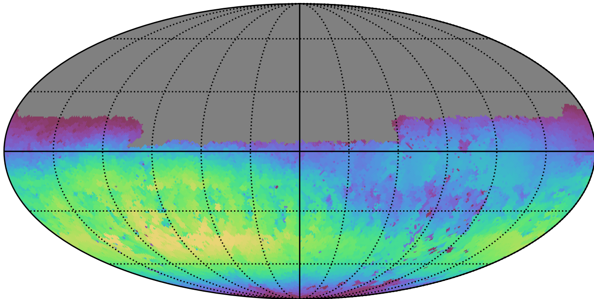
no_long_daily_v3.4_10yrs Yr 1 u band: Max skyBrightness
