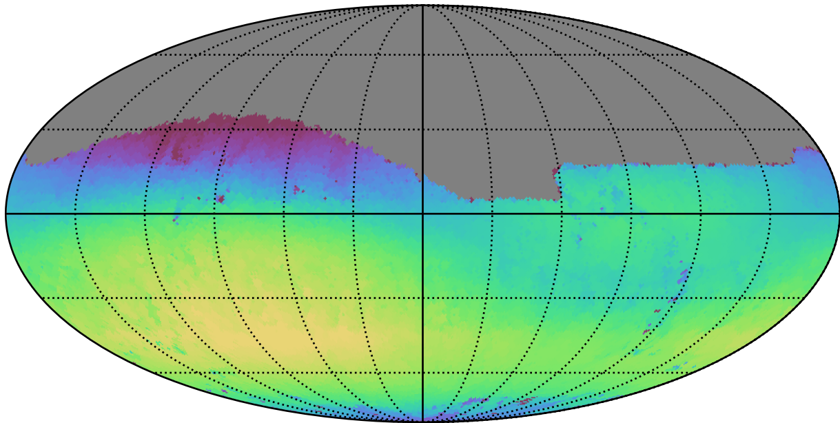
no_long_daily_v3.4_10yrs Yr 1 r band: Max skyBrightness
