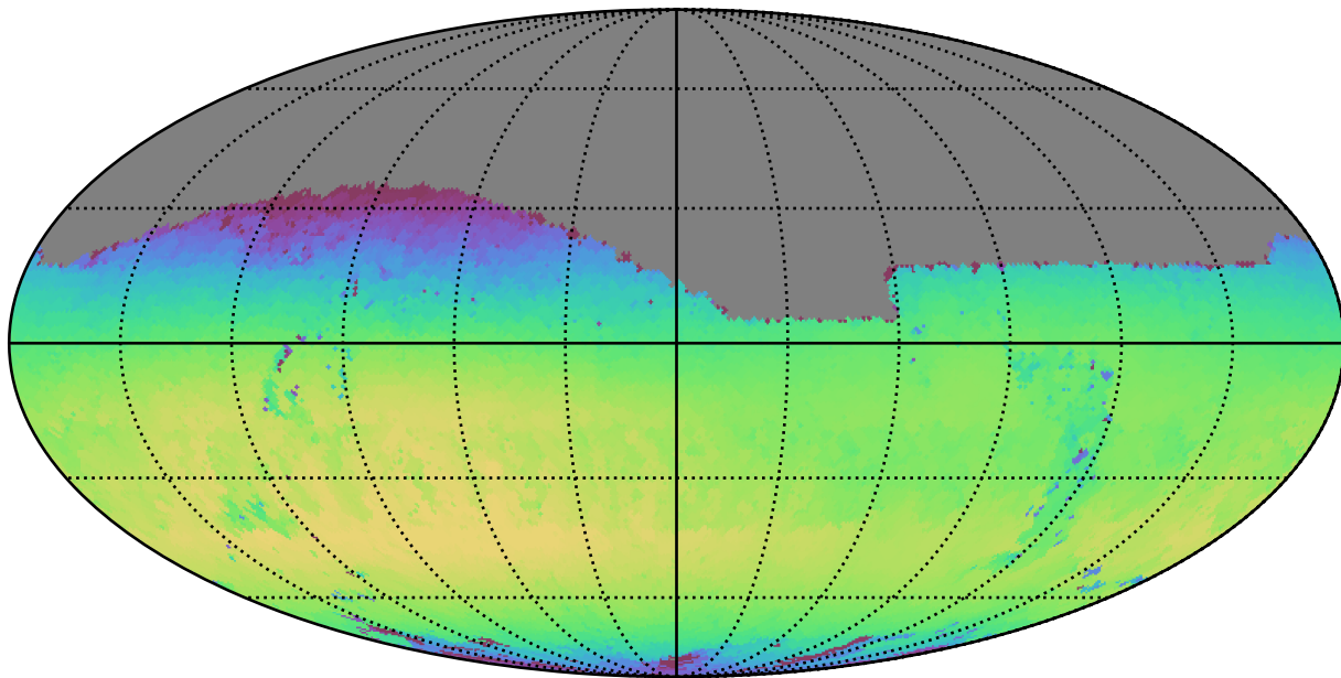
no_long_daily_v3.4_10yrs Yr 1 i band: Max skyBrightness
