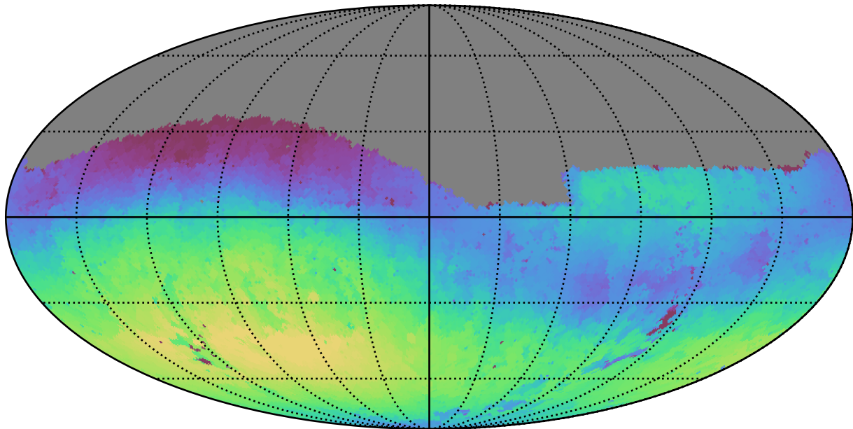
no_long_daily_v3.4_10yrs Yr 1 g band: Max skyBrightness
