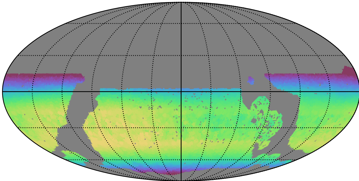
no_long_daily_v3.4_10yrs WFD z band: Max skyBrightness
