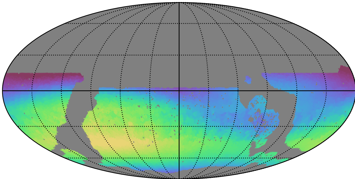
no_long_daily_v3.4_10yrs WFD u band: Max skyBrightness
