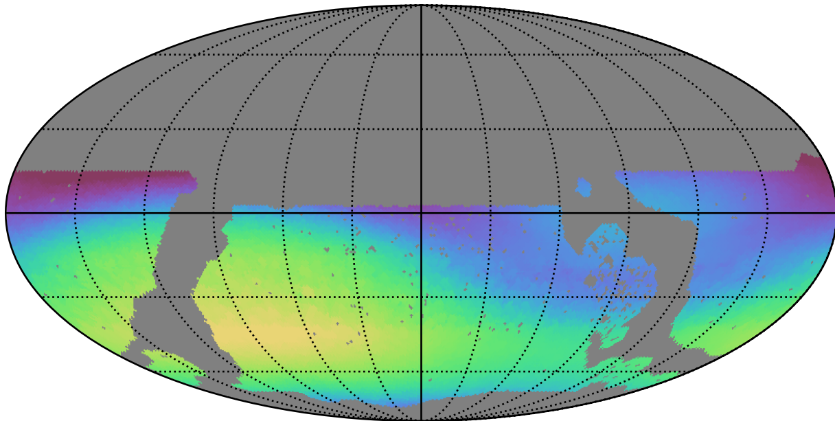
no_long_daily_v3.4_10yrs WFD r band: Max skyBrightness
