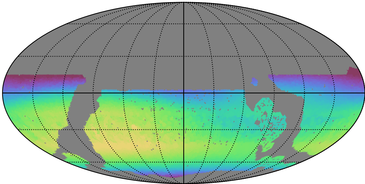
no_long_daily_v3.4_10yrs WFD i band: Max skyBrightness
