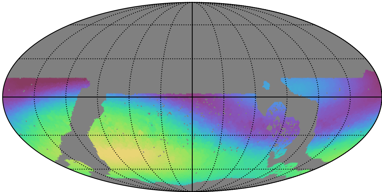
no_long_daily_v3.4_10yrs WFD g band: Max skyBrightness
