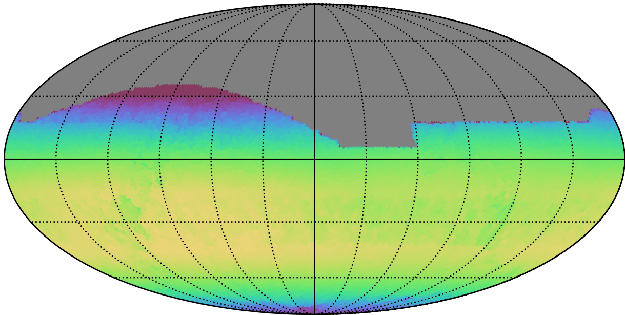
no_long_daily_v3.4_10yrs All sky z band: Max skyBrightness
