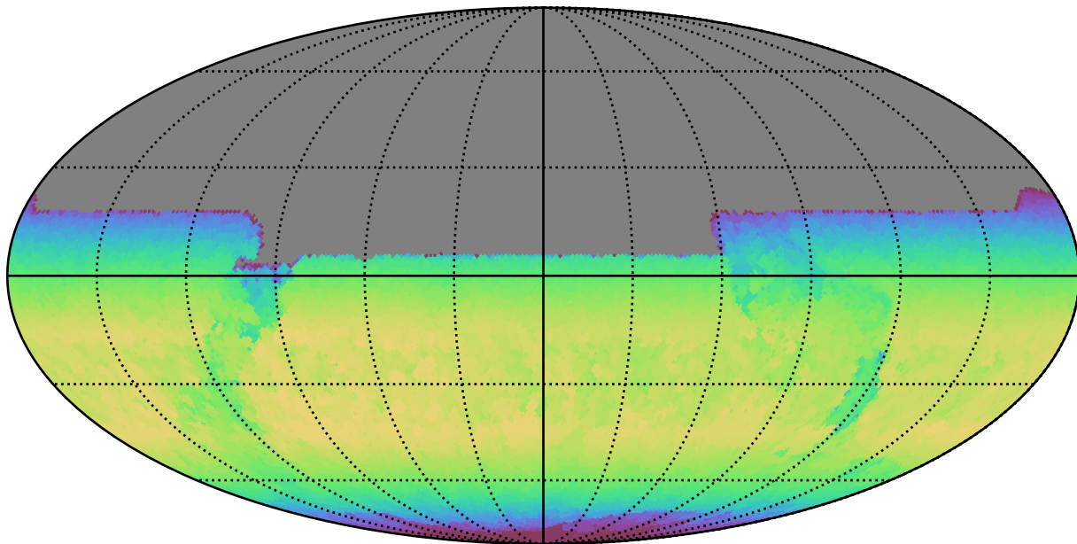
no_long_daily_v3.4_10yrs All sky y band: Max skyBrightness
