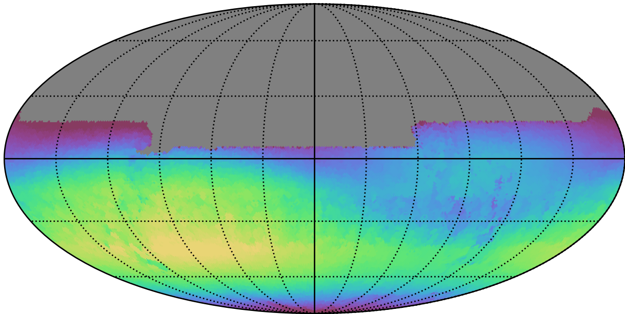
no_long_daily_v3.4_10yrs All sky u band: Max skyBrightness
