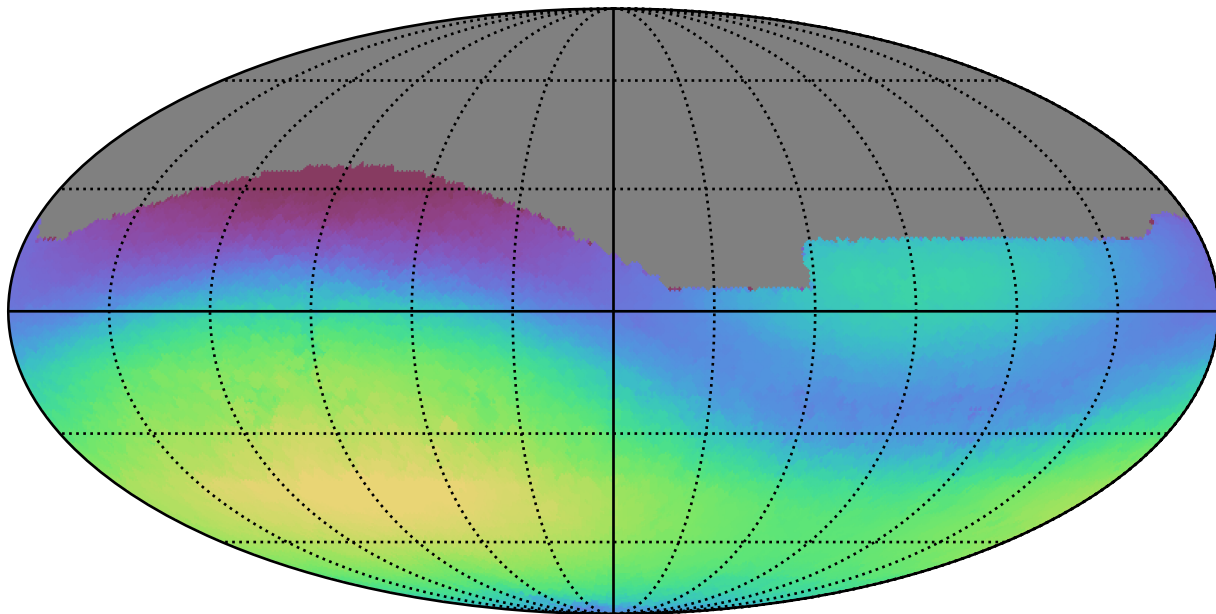
no_long_daily_v3.4_10yrs All sky g band: Max skyBrightness
