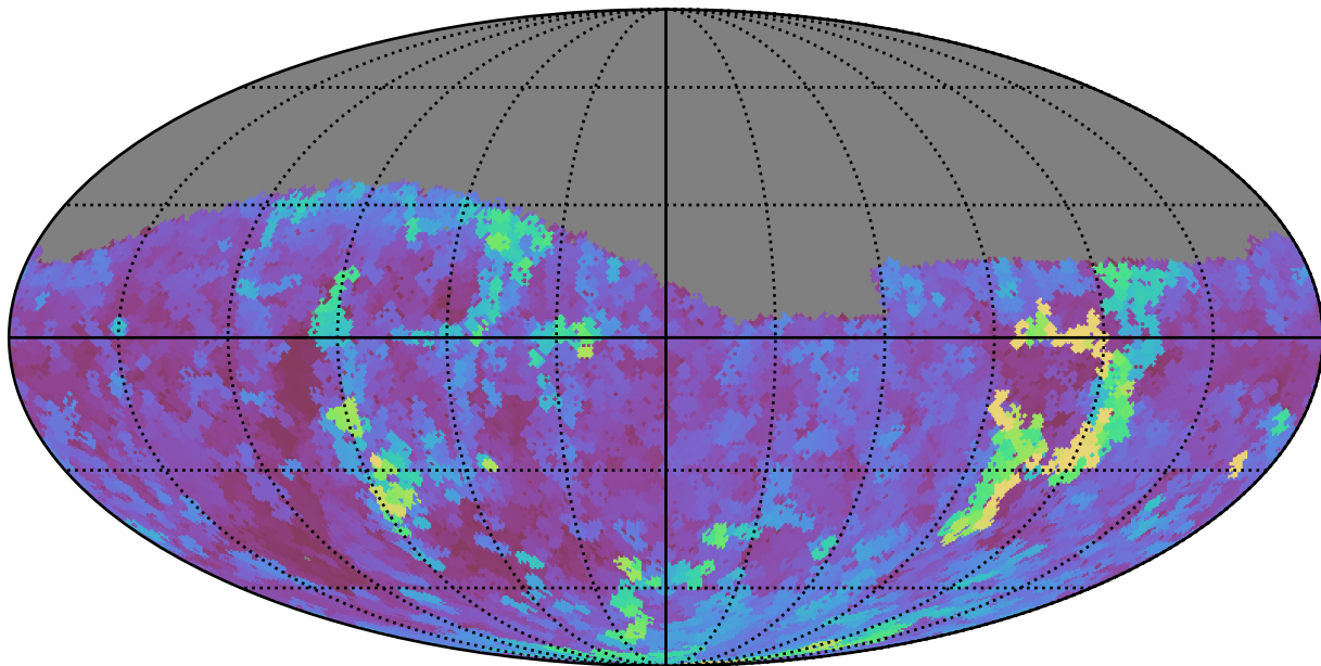
no_long_daily_v3.4_10yrs Yr 1 g band: Max seeingEff
