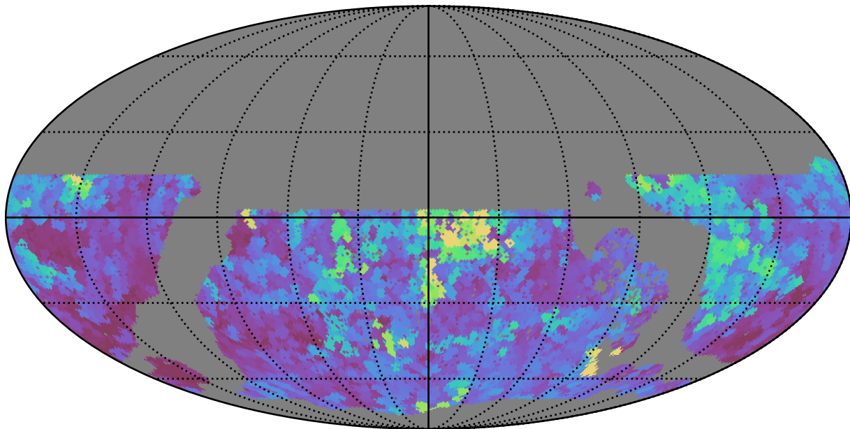
no_long_daily_v3.4_10yrs WFD z band: Max seeingEff
