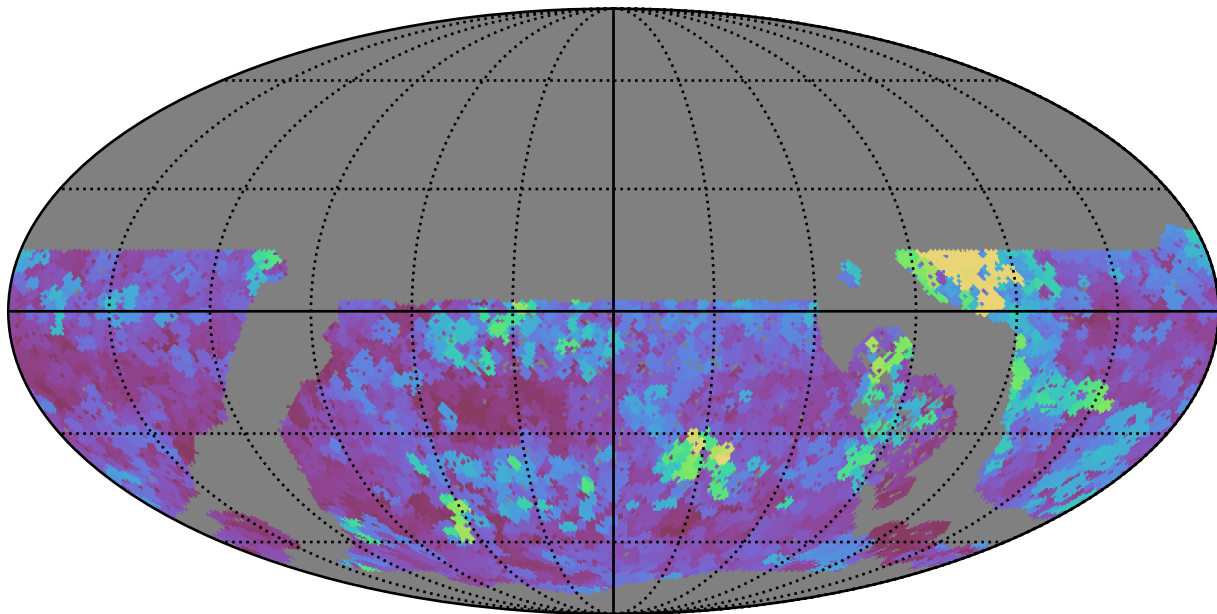
no_long_daily_v3.4_10yrs WFD u band: Max seeingEff
