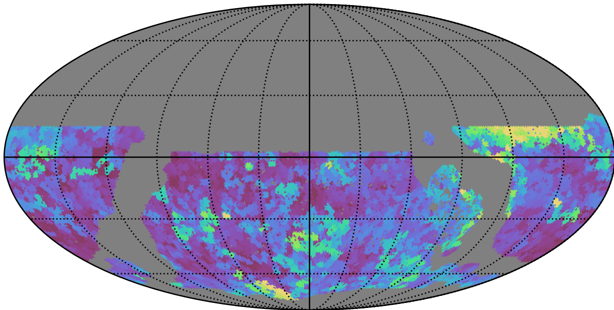
no_long_daily_v3.4_10yrs WFD g band: Max seeingEff
