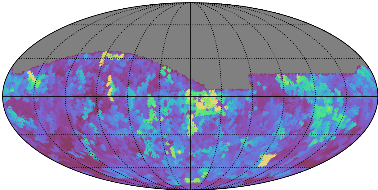
no_long_daily_v3.4_10yrs All sky z band: Max seeingEff
