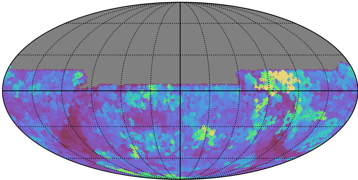
no_long_daily_v3.4_10yrs All sky u band: Max seeingEff
