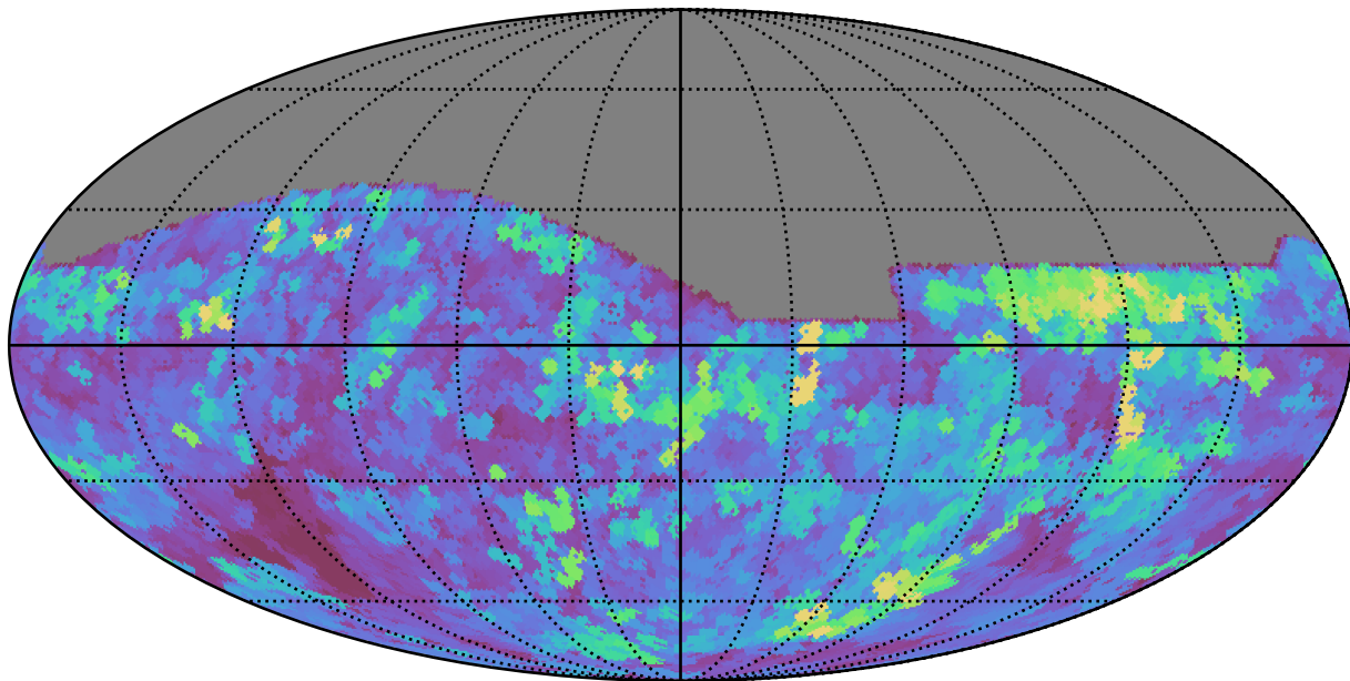
no_long_daily_v3.4_10yrs All sky r band: Max seeingEff
