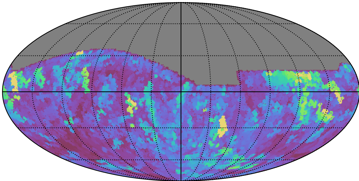
no_long_daily_v3.4_10yrs All sky i band: Max seeingEff
