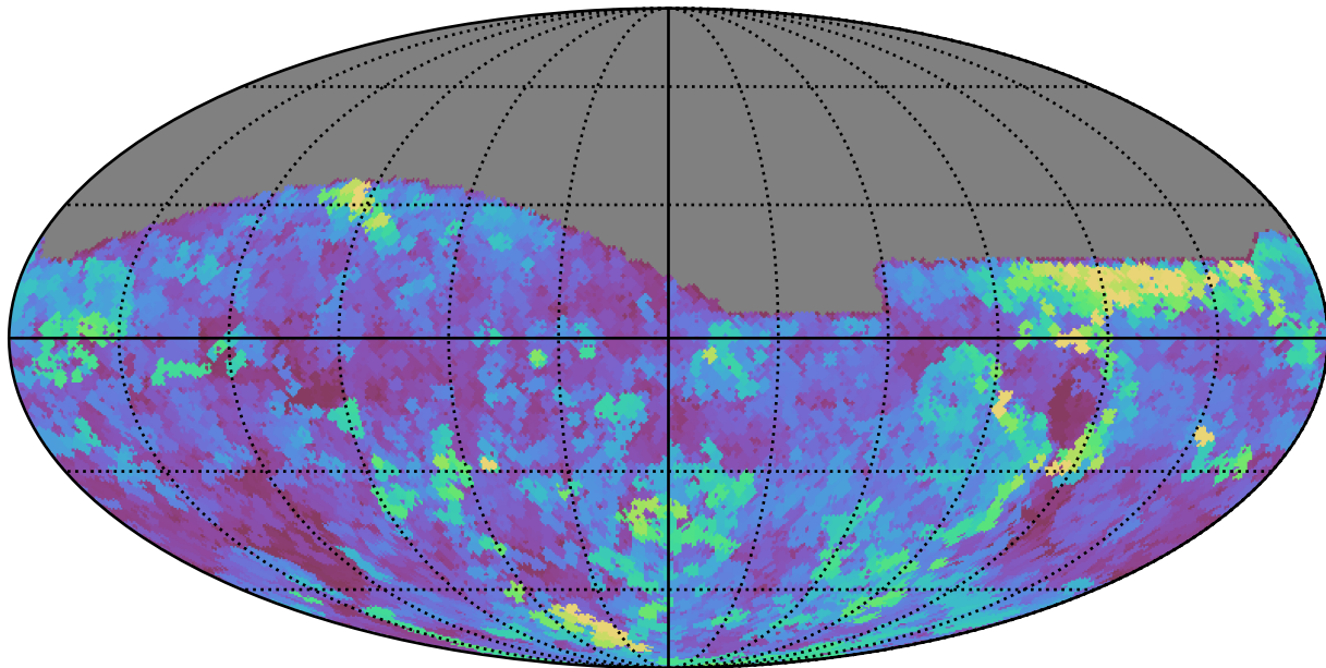
no_long_daily_v3.4_10yrs All sky g band: Max seeingEff
