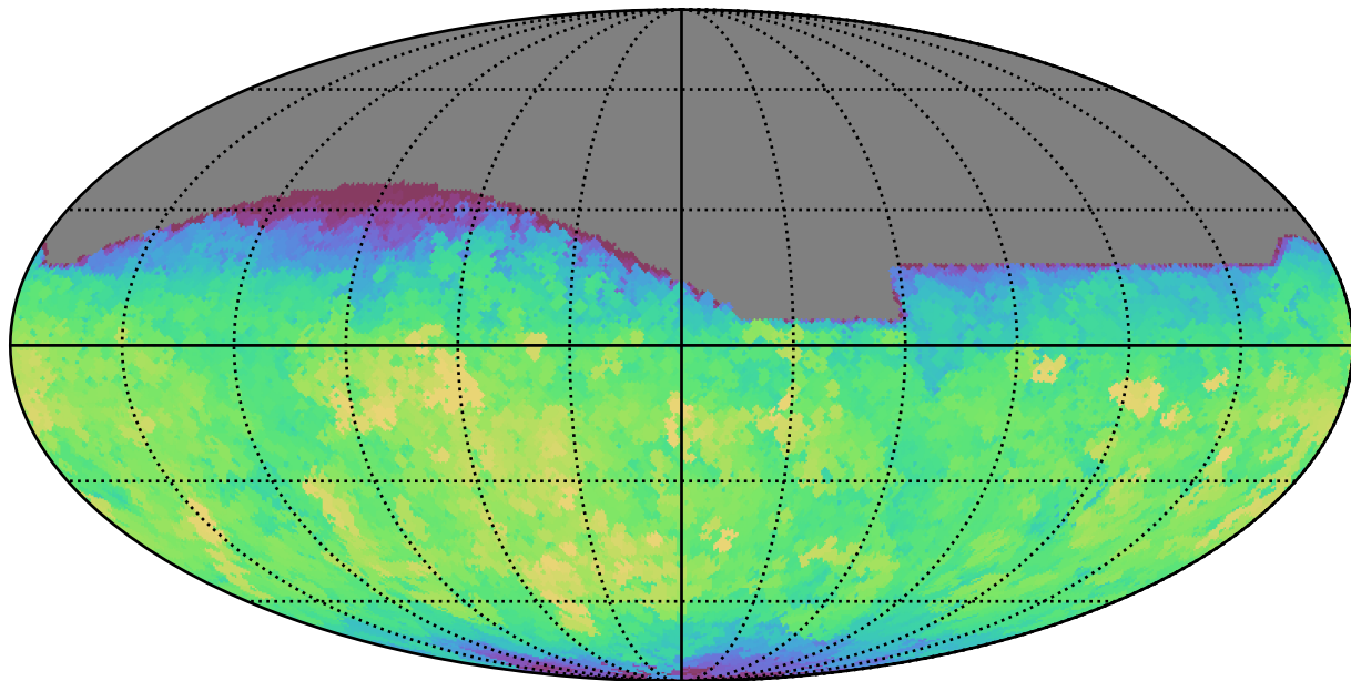
no_long_daily_v3.4_10yrs All sky all bands: Max saturation_mag
