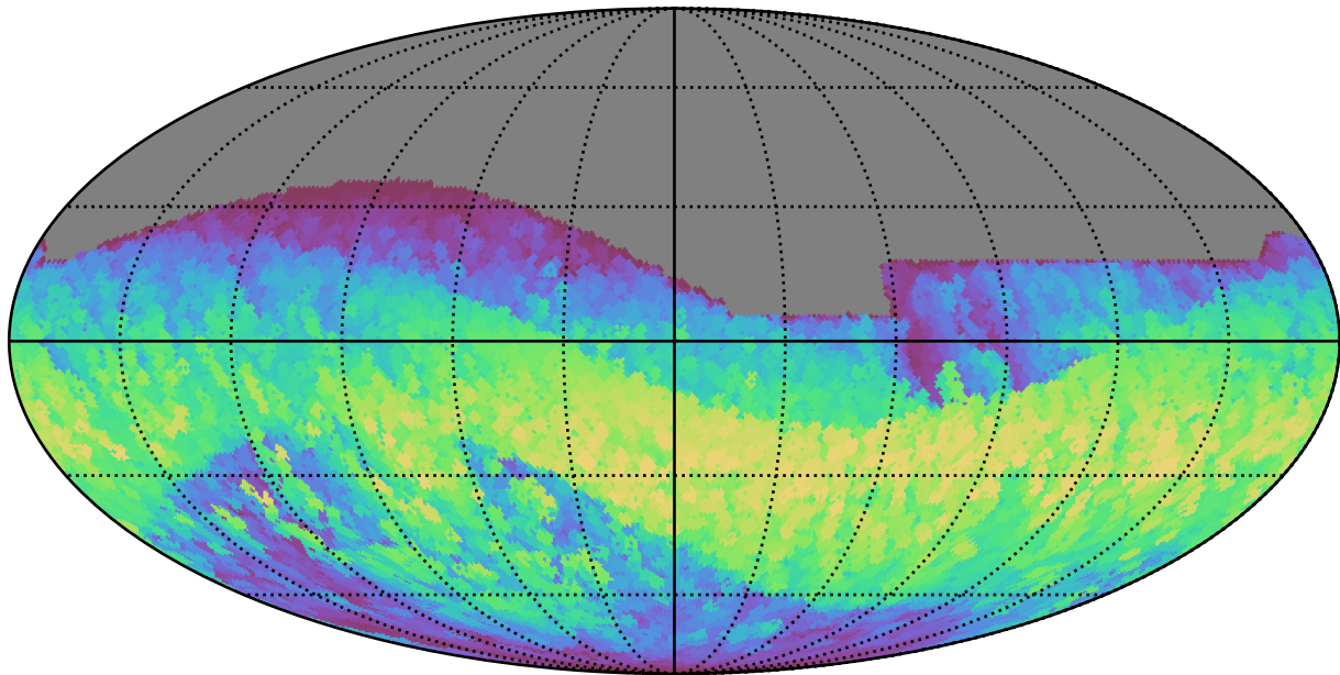
no_long_daily_v3.4_10yrs All sky all bands: Max normairmass
