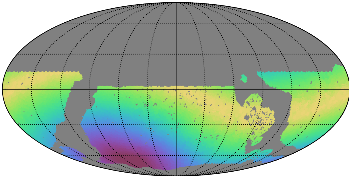
no_long_daily_v3.4_10yrs WFD all bands: Max moonDistance
