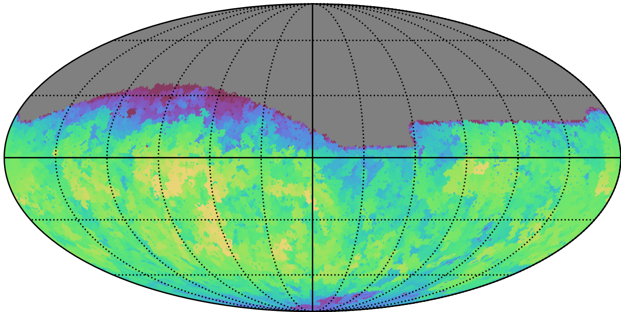
no_long_daily_v3.4_10yrs Yr 1 all bands: Max fiveSigmaDepth
