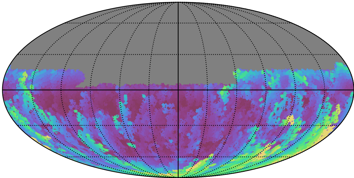
no_long_daily_v3.4_10yrs Yr 1 u band: Max airmass
