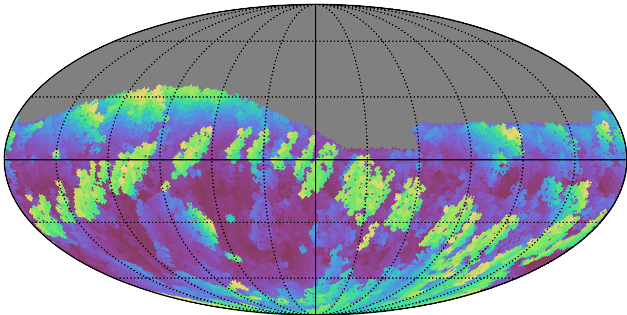
no_long_daily_v3.4_10yrs Yr 1 r band: Max airmass
