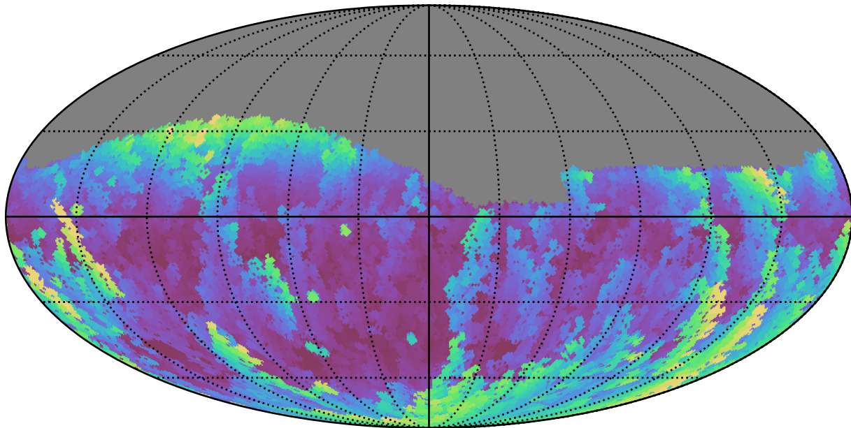
no_long_daily_v3.4_10yrs Yr 1 g band: Max airmass
