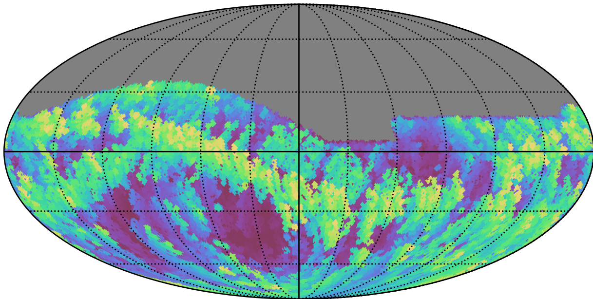
no_long_daily_v3.4_10yrs Yr 1 all bands: Max airmass
