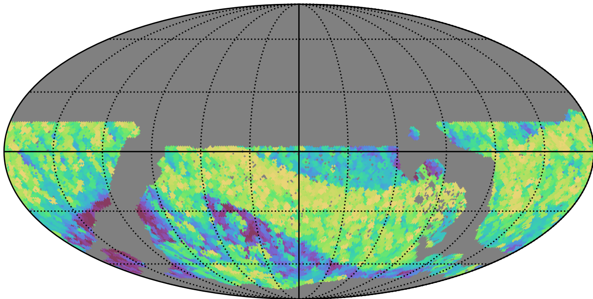
no_long_daily_v3.4_10yrs WFD all bands: Max airmass
