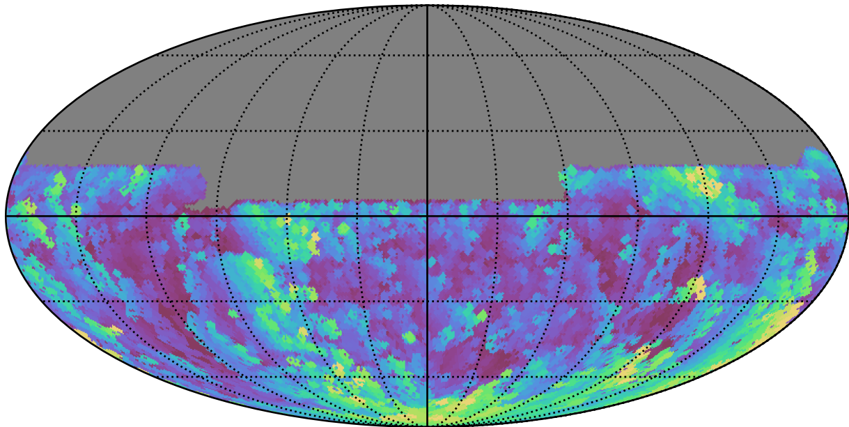
no_long_daily_v3.4_10yrs All sky u band: Max airmass
