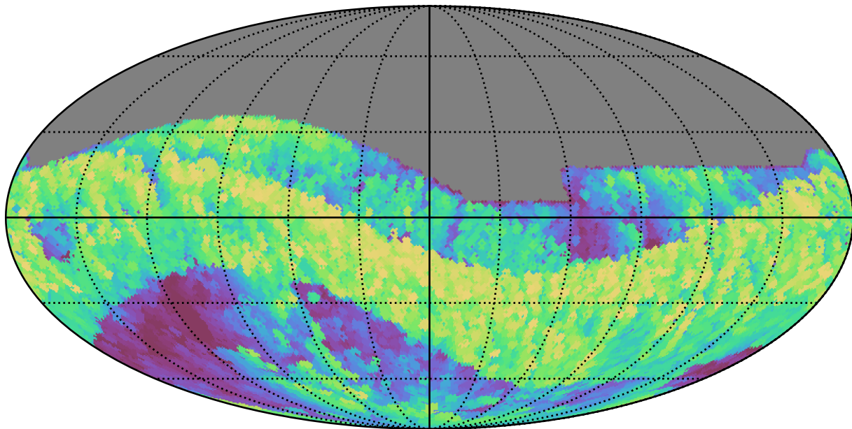
no_long_daily_v3.4_10yrs All sky i band: Max airmass
