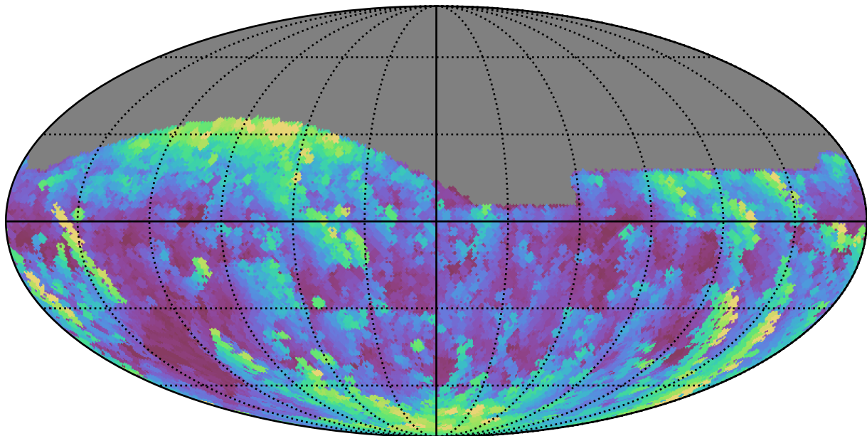
no_long_daily_v3.4_10yrs All sky g band: Max airmass
