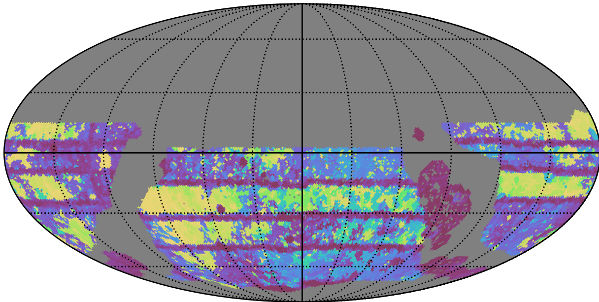
no_long_daily_v3.4_10yrs WFD z band: Max Inter-Night Gap
