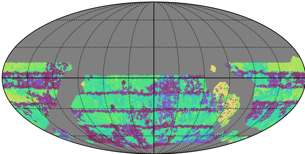
no_long_daily_v3.4_10yrs WFD u band: Max Inter-Night Gap
