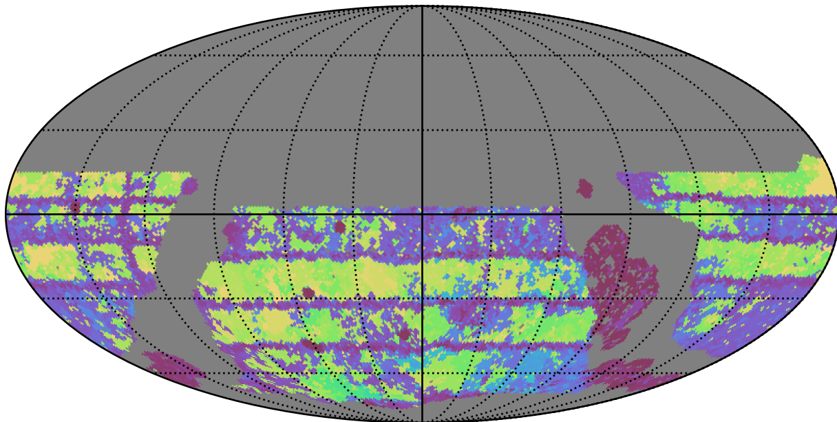
no_long_daily_v3.4_10yrs WFD g band: Max Inter-Night Gap
