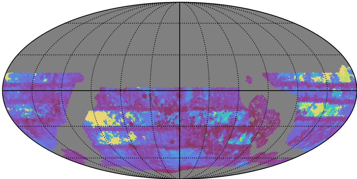
no_long_daily_v3.4_10yrs WFD all bands: Max Inter-Night Gap
