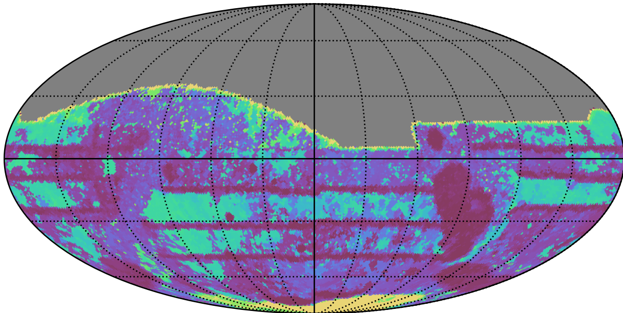
no_long_daily_v3.4_10yrs All sky z band: Max Inter-Night Gap
