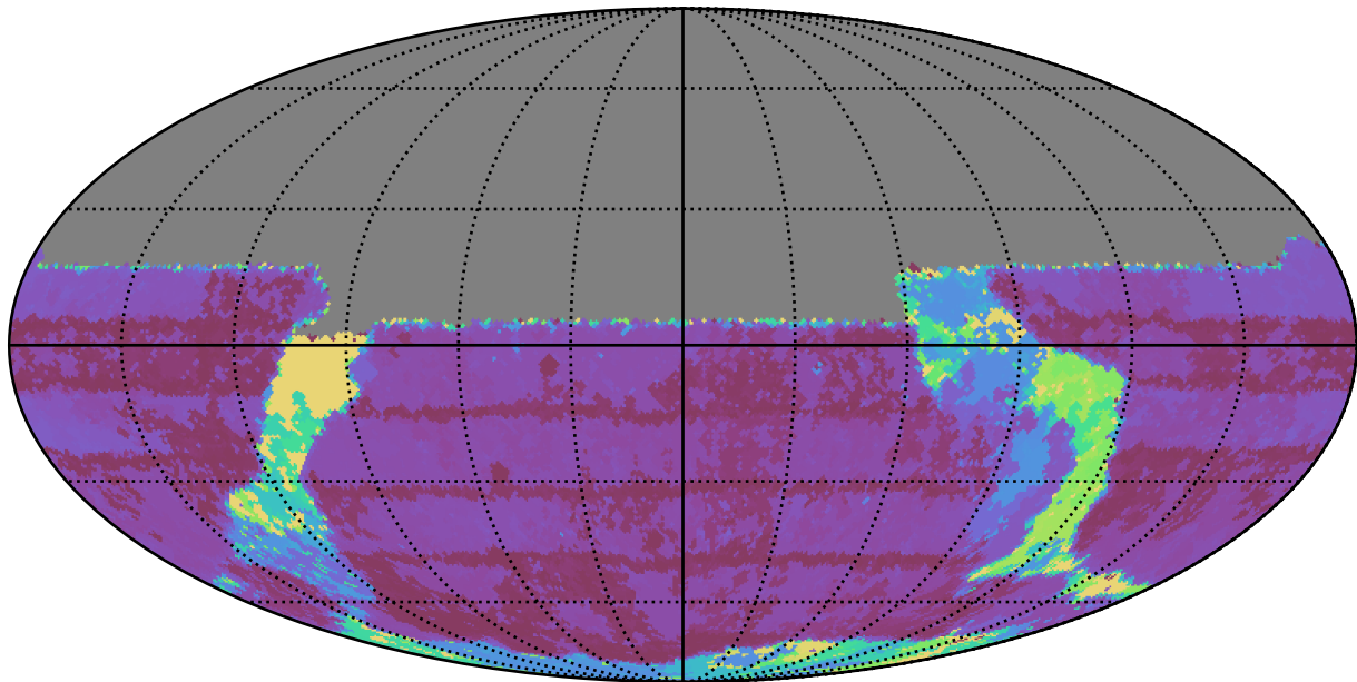
no_long_daily_v3.4_10yrs All sky u band: Max Inter-Night Gap
