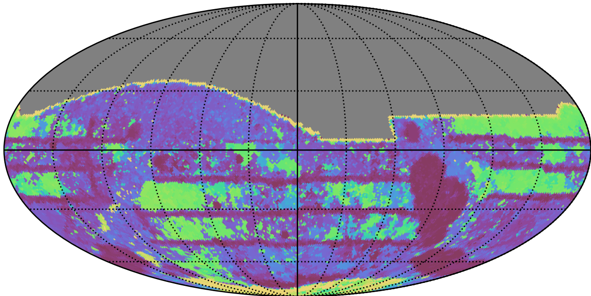
no_long_daily_v3.4_10yrs All sky i band: Max Inter-Night Gap
