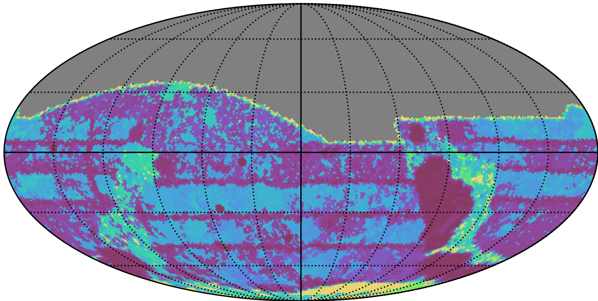
no_long_daily_v3.4_10yrs All sky g band: Max Inter-Night Gap
