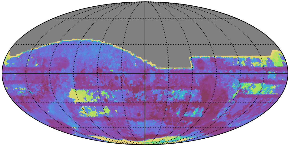
no_long_daily_v3.4_10yrs All sky all bands: Max Inter-Night Gap
