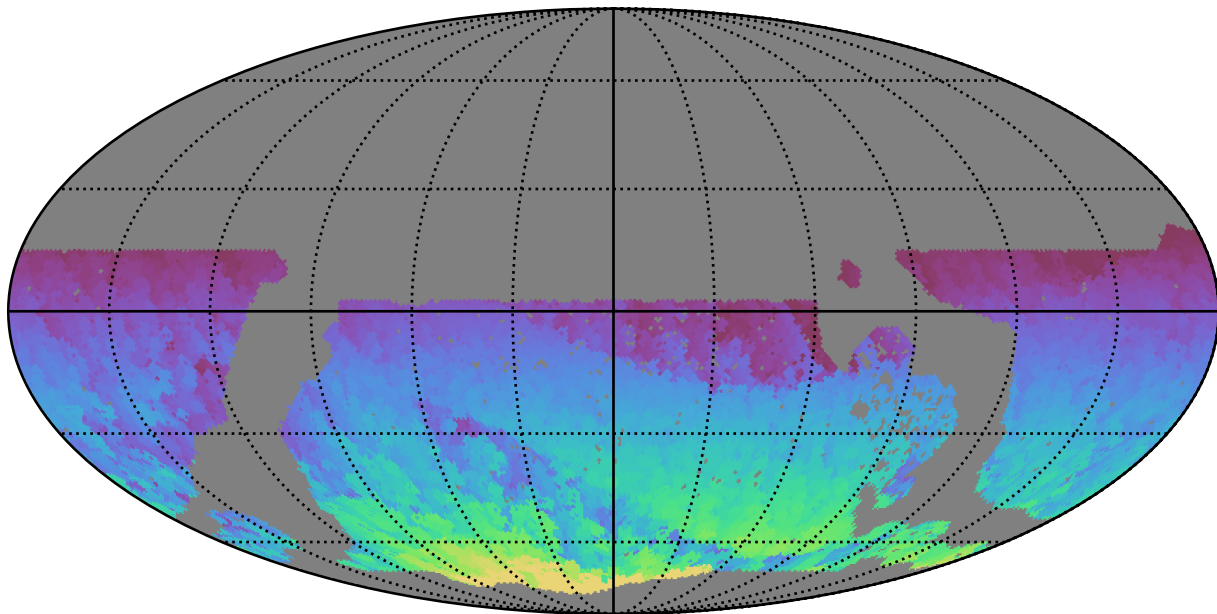
no_long_daily_v3.4_10yrs WFD all bands: Max HA
