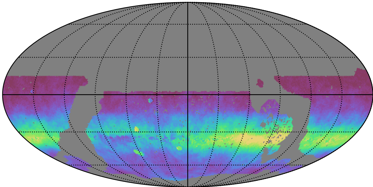
no_long_daily_v3.4_10yrs WFD all bands: AngleRms rotSkyPos
