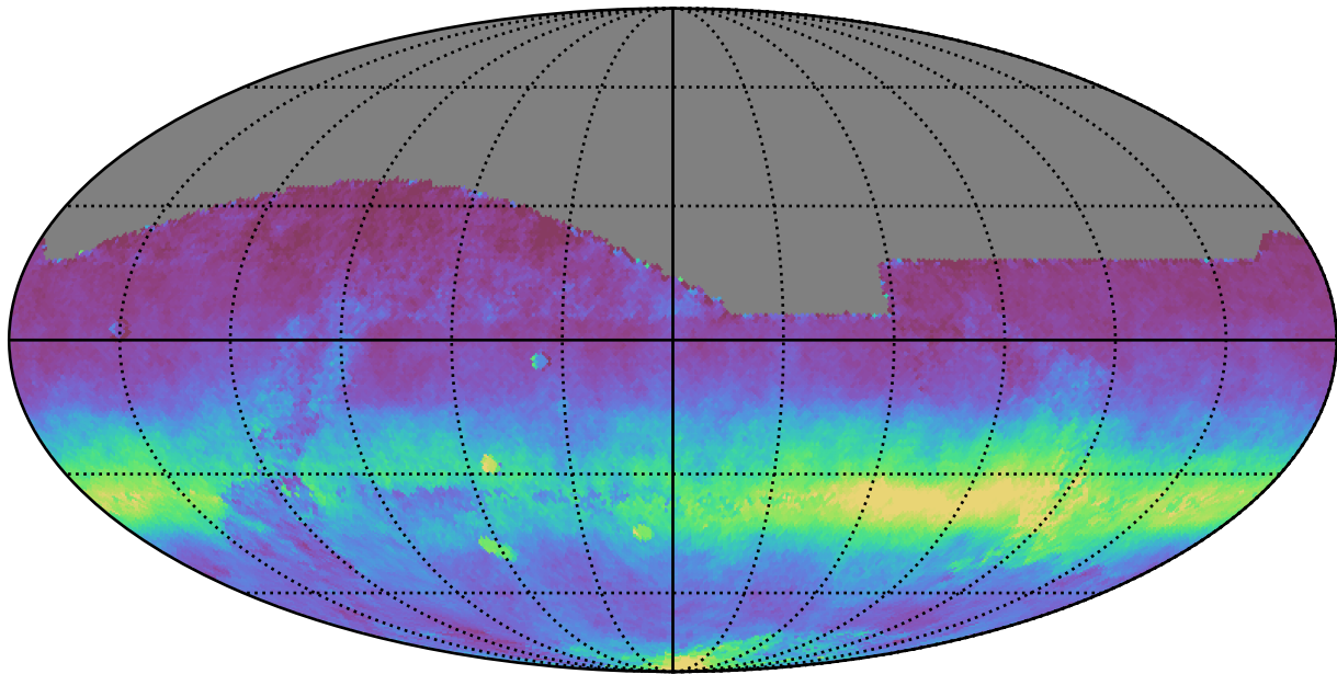
no_long_daily_v3.4_10yrs All sky all bands: AngleRms rotSkyPos
