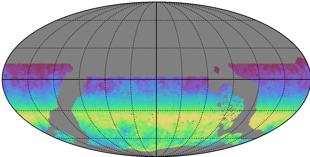
no_long_daily_v3.4_10yrs WFD all bands: AngleRange rotSkyPos
