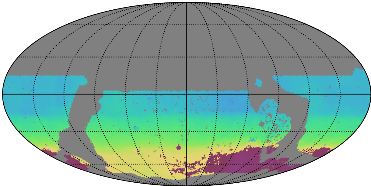
no_long_daily_v3.4_10yrs WFD all bands: AngleMean rotSkyPos
