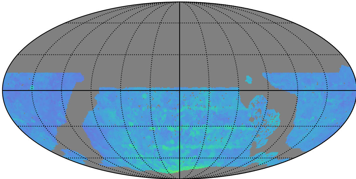
no_long_daily_v3.4_10yrs WFD z band: 80thPercentile Season Length
