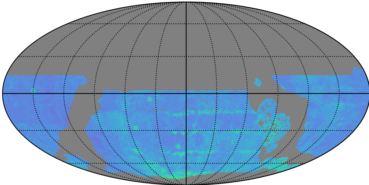
no_long_daily_v3.4_10yrs WFD r band: 80thPercentile Season Length
